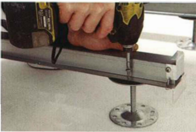
4. Fixing Pillars and joists
